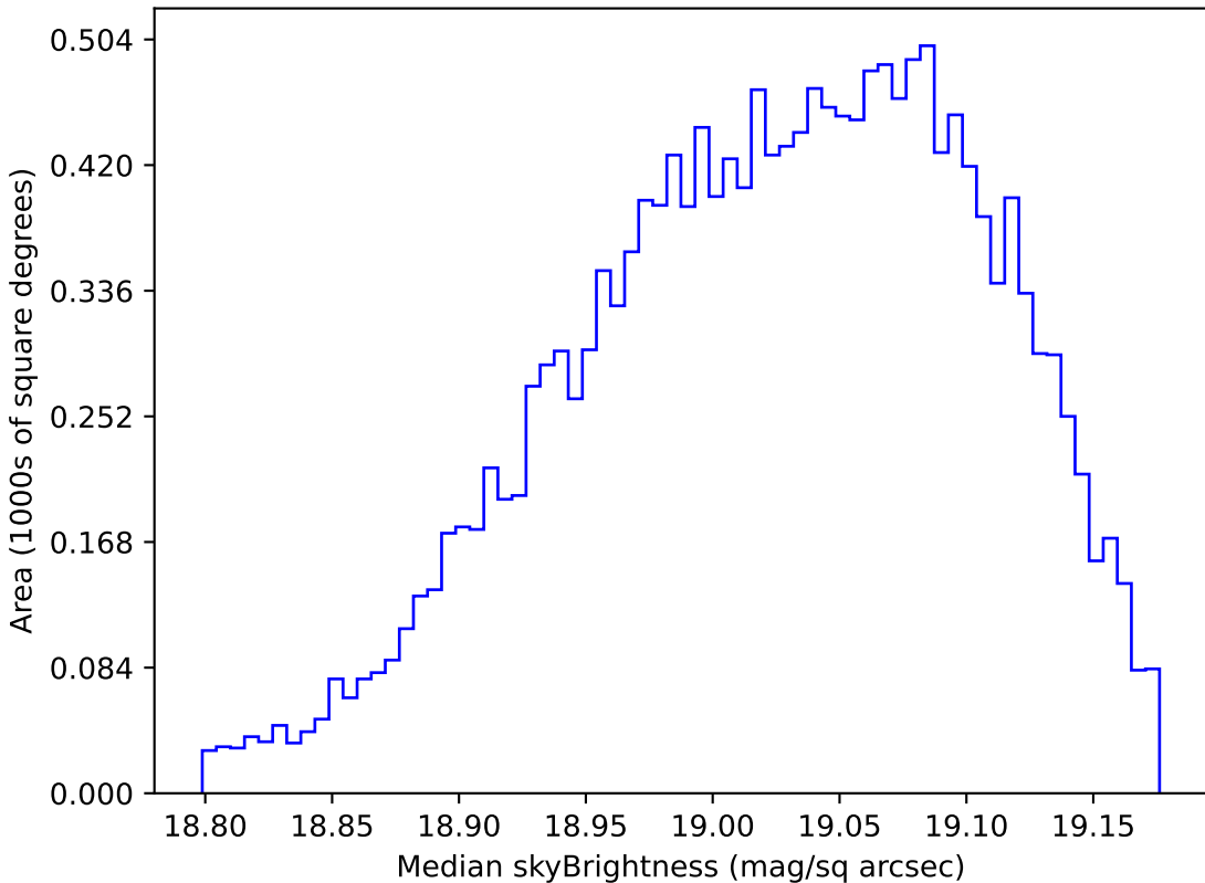
internal_u_expt60_nscale0.9v3.4_10yrs WFD z band: Median skyBrightness
