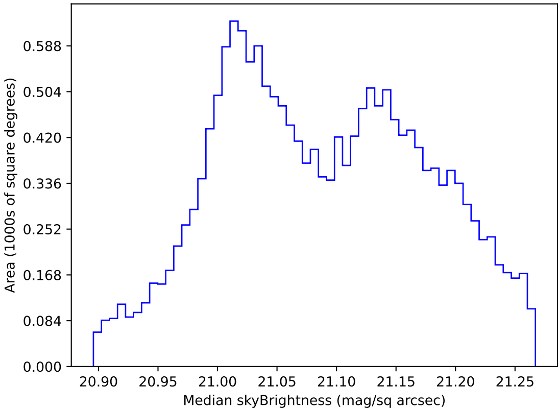
internal_u_expt60_nscale0.9v3.4_10yrs WFD r band: Median skyBrightness
