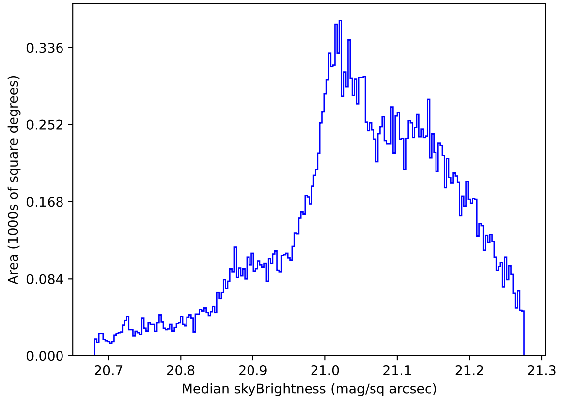
internal_u_expt60_nscale0.9v3.4_10yrs All sky r band: Median skyBrightness
