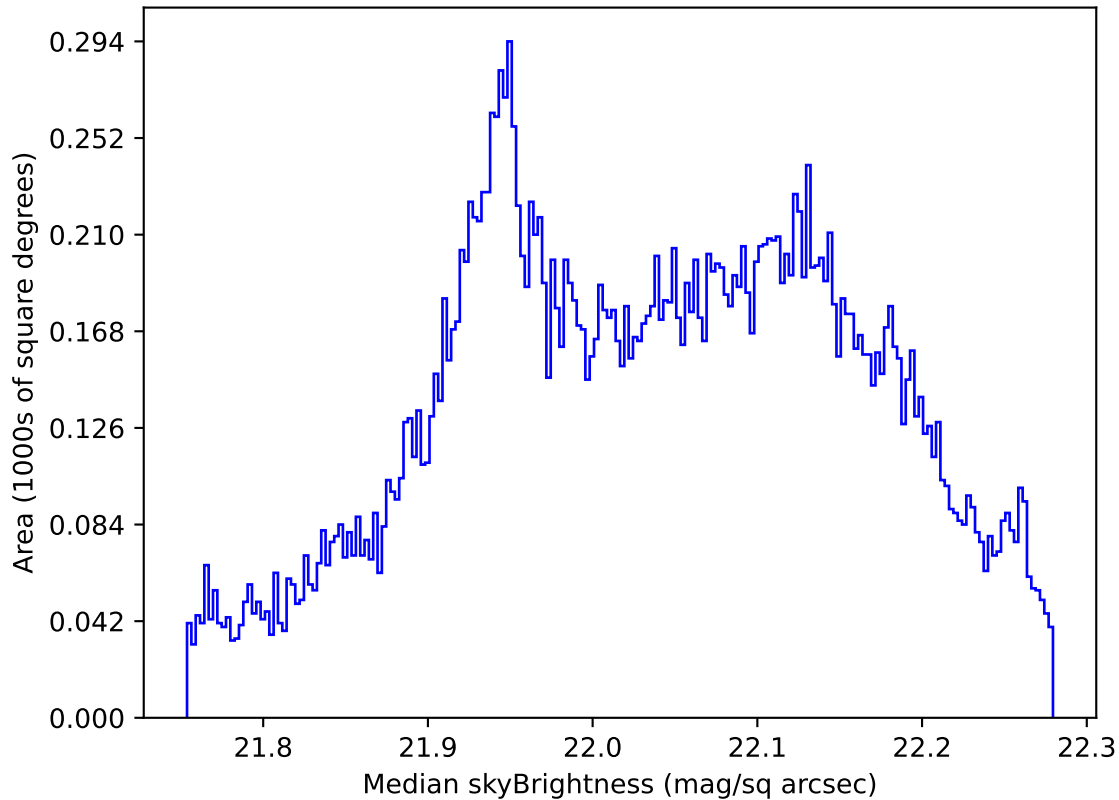
internal_u_expt60_nscale0.9v3.4_10yrs All sky g band: Median skyBrightness
