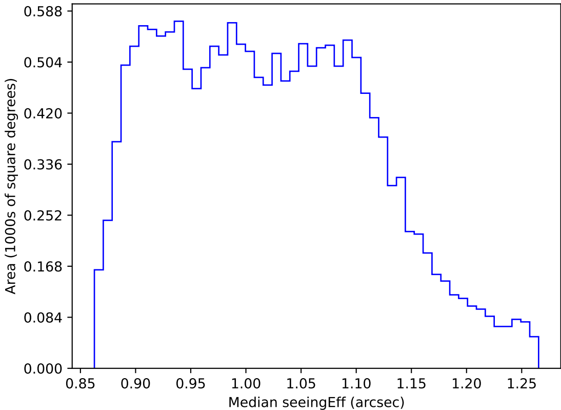
internal_u_expt60_nscale0.9v3.4_10yrs WFD r band: Median seeingEff
