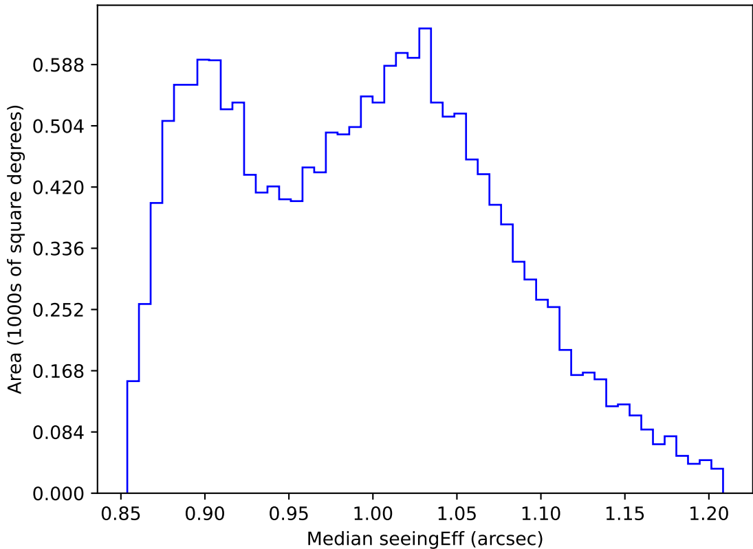
internal_u_expt60_nscale0.9v3.4_10yrs WFD i band: Median seeingEff
