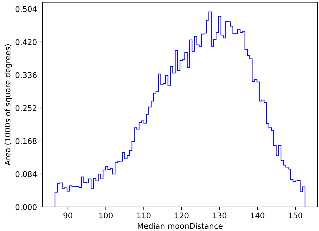
internal_u_expt60_nscale0.9v3.4_10yrs All sky u band: Median moonDistance
