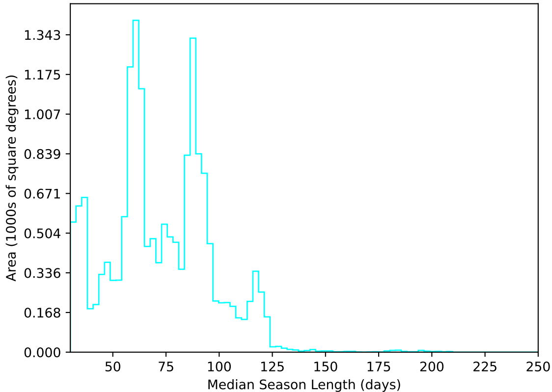
internal_u_expt60_nscale0.9v3.4_10yrs WFD u band: Median Season Length
