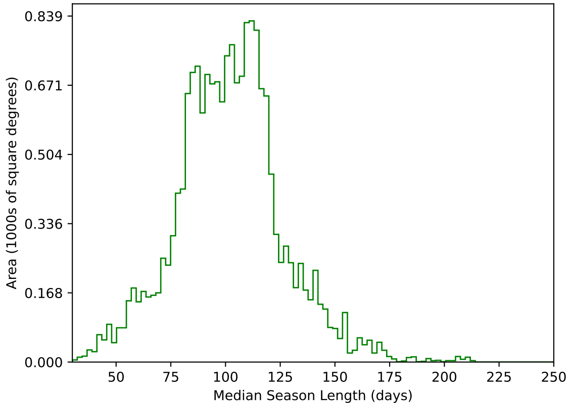
internal_u_expt60_nscale0.9v3.4_10yrs WFD g band: Median Season Length
