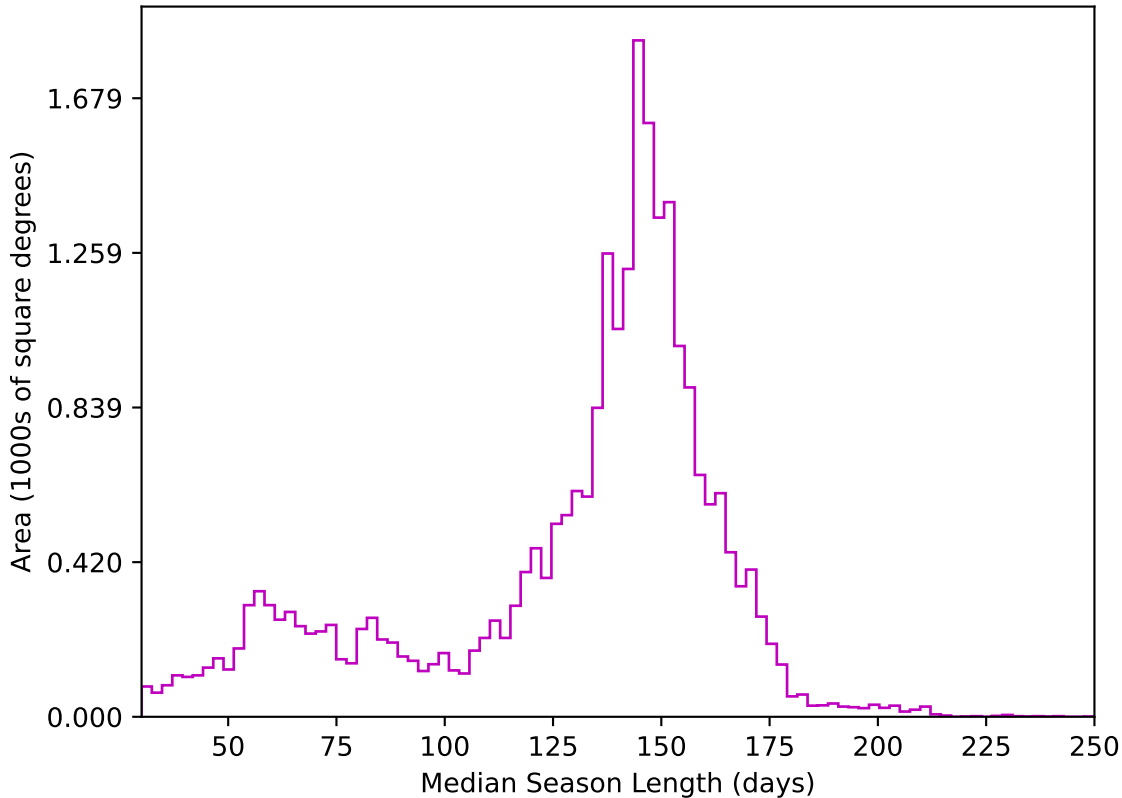
internal_u_expt60_nscale0.9v3.4_10yrs All sky z band: Median Season Length
