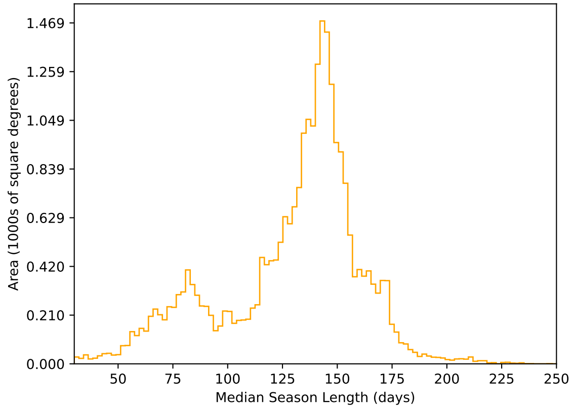
internal_u_expt60_nscale0.9v3.4_10yrs All sky r band: Median Season Length
