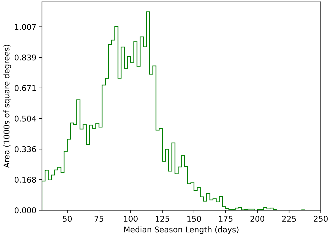
internal_u_expt60_nscale0.9v3.4_10yrs All sky g band: Median Season Length
