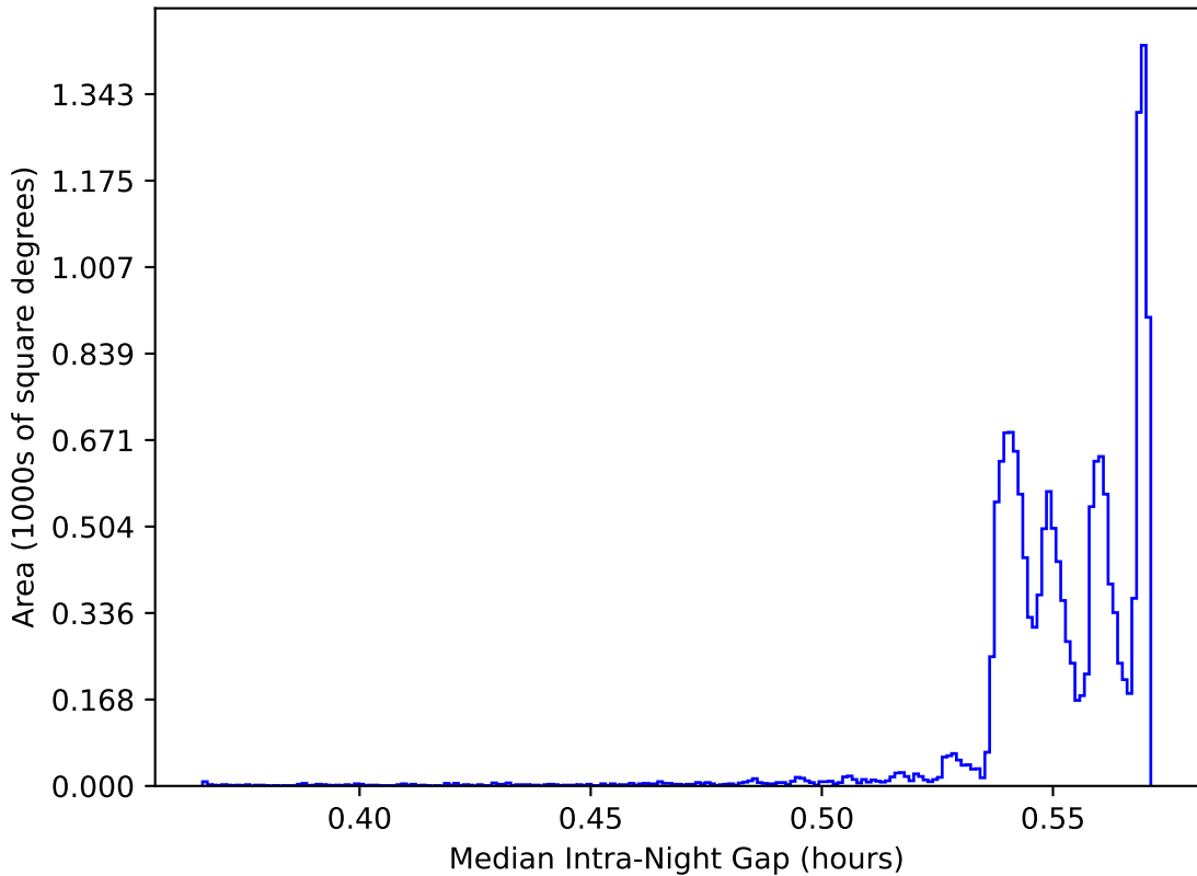
internal_u_expt60_nscale0.9v3.4_10yrs WFD: Median Intra-Night Gap
