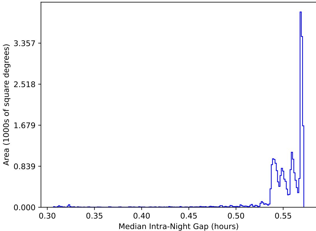
internal_u_expt60_nscale0.9v3.4_10yrs All sky: Median Intra-Night Gap
