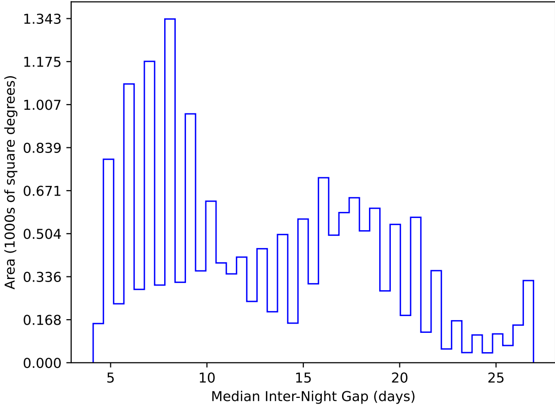
internal_u_expt60_nscale0.9v3.4_10yrs WFD y band: Median Inter-Night Gap
