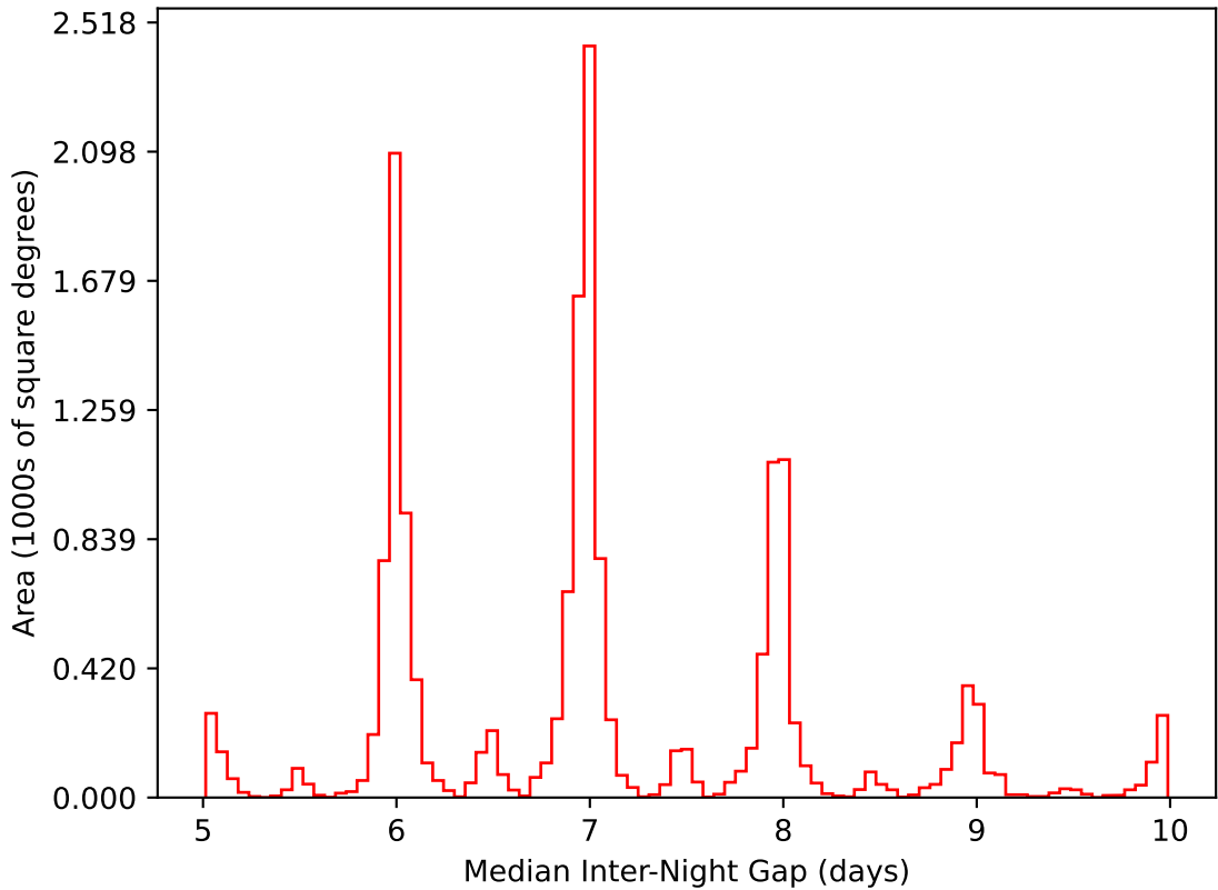
internal_u_expt60_nscale0.9v3.4_10yrs WFD i band: Median Inter-Night Gap
