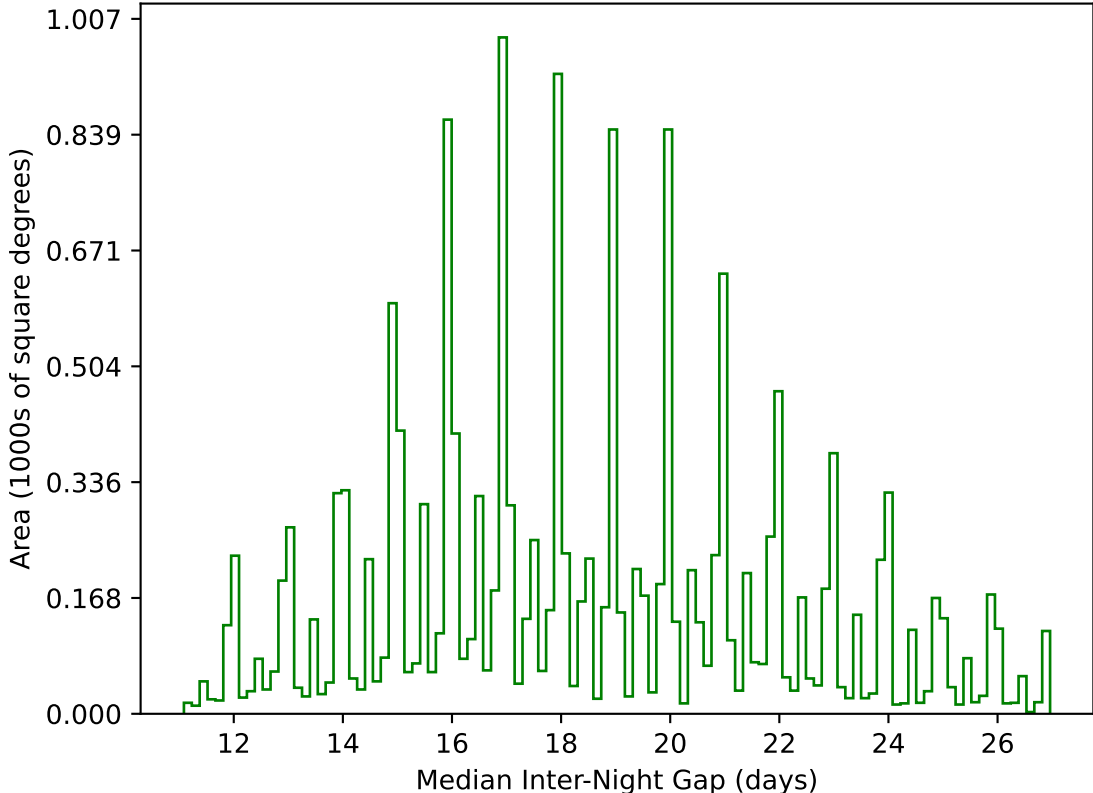
internal_u_expt60_nscale0.9v3.4_10yrs WFD g band: Median Inter-Night Gap
