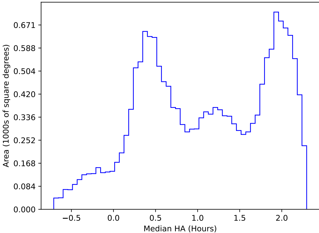
internal_u_expt60_nscale0.9v3.4_10yrs WFD z band: Median HA
