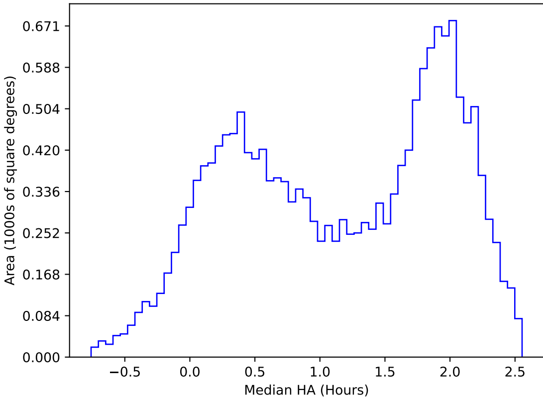
internal_u_expt60_nscale0.9v3.4_10yrs WFD u band: Median HA
