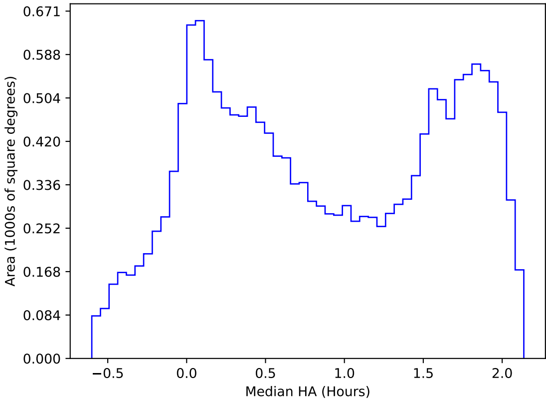
internal_u_expt60_nscale0.9v3.4_10yrs WFD r band: Median HA
