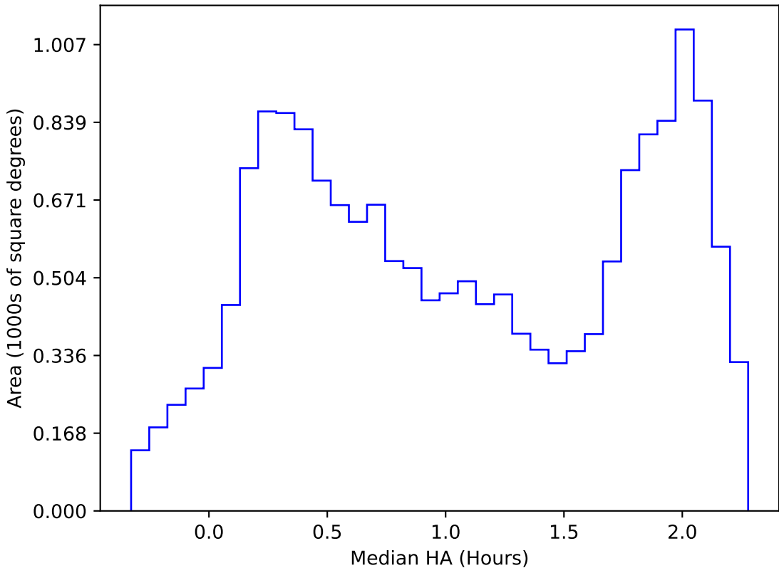
internal_u_expt60_nscale0.9v3.4_10yrs WFD i band: Median HA
