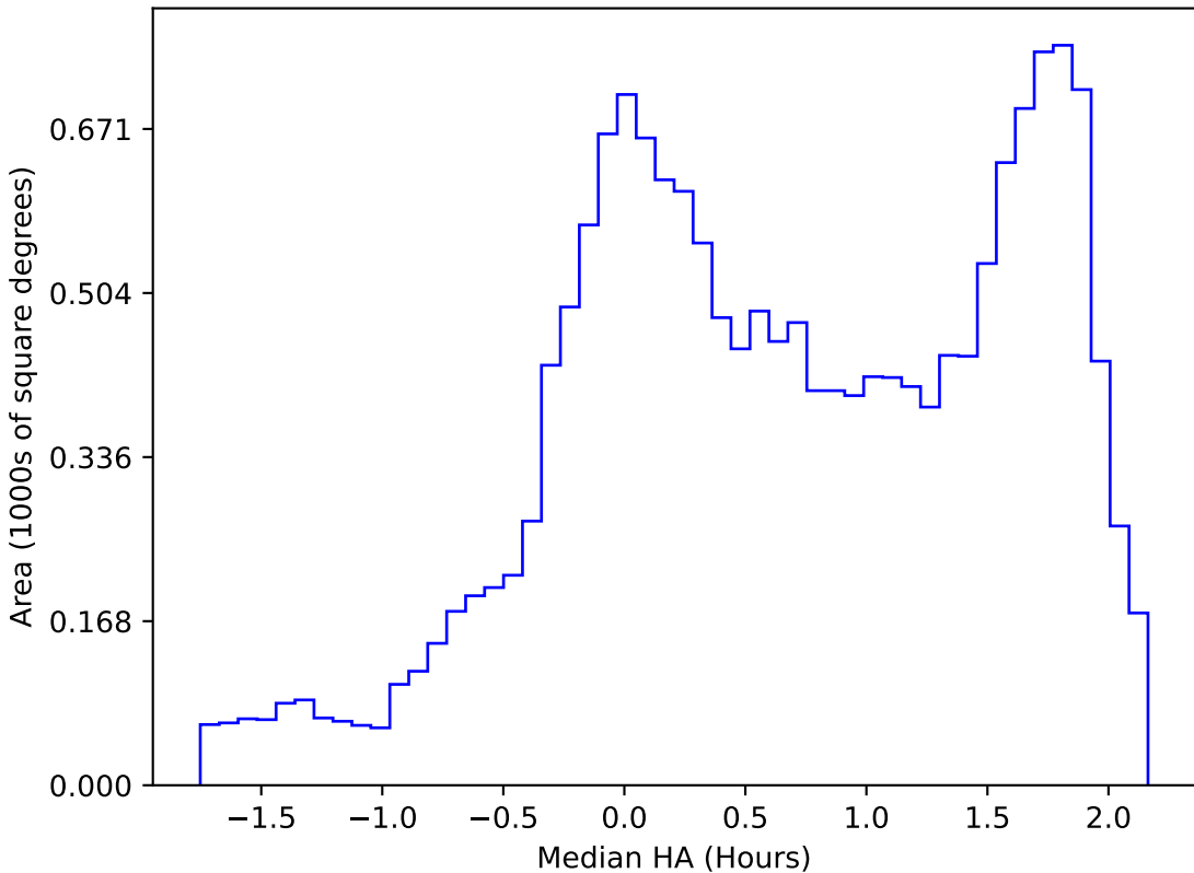
internal_u_expt60_nscale0.9v3.4_10yrs WFD g band: Median HA
