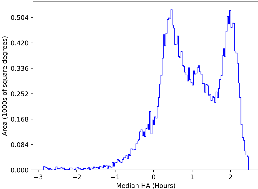
internal_u_expt60_nscale0.9v3.4_10yrs All sky z band: Median HA
