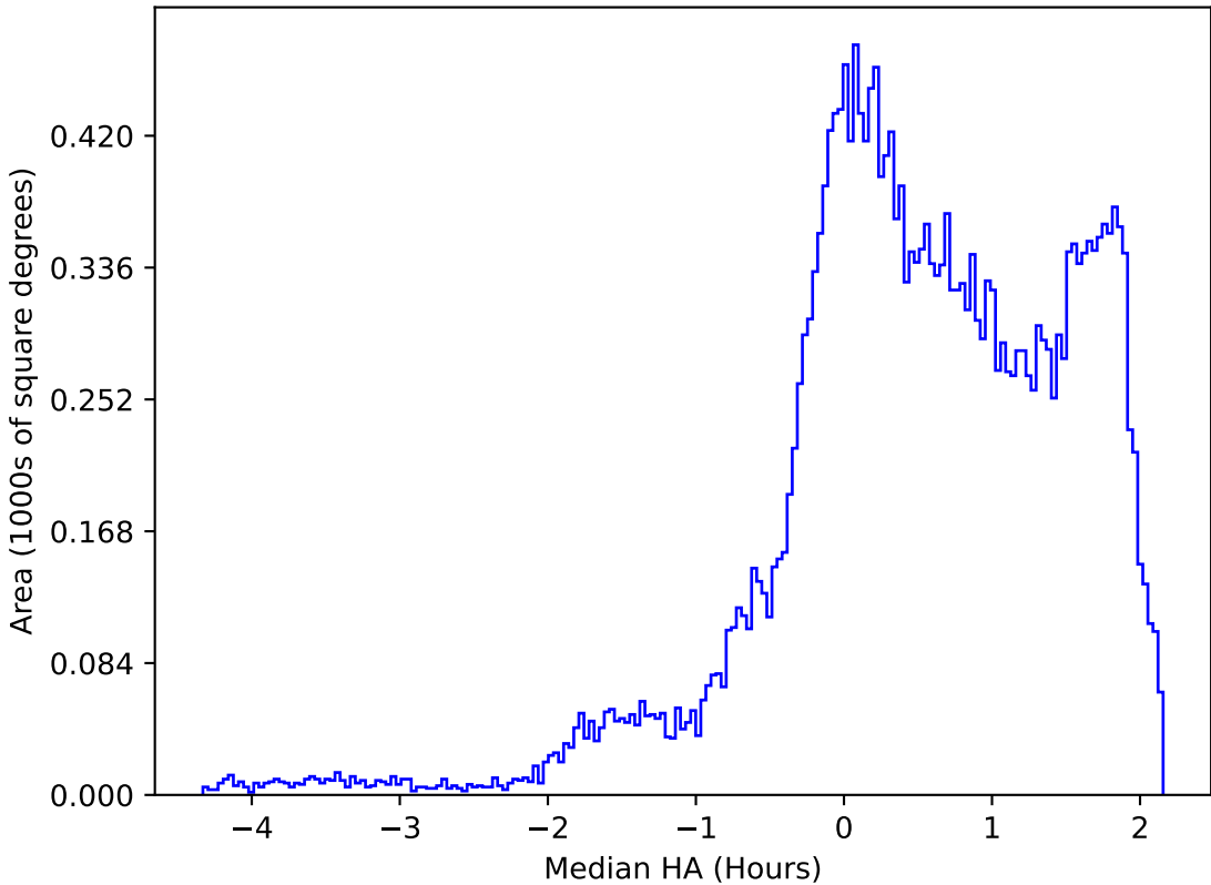
internal_u_expt60_nscale0.9v3.4_10yrs All sky g band: Median HA
