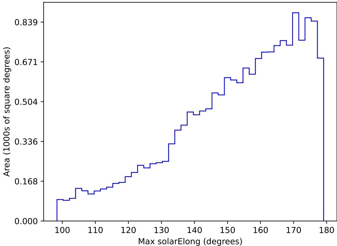
internal_u_expt60_nscale0.9v3.4_10yrs WFD u band: Max solarElong
