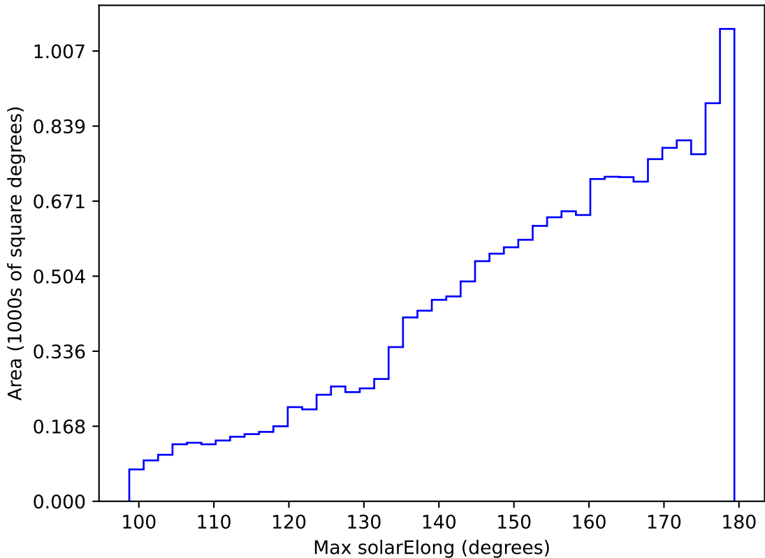
internal_u_expt60_nscale0.9v3.4_10yrs WFD i band: Max solarElong
