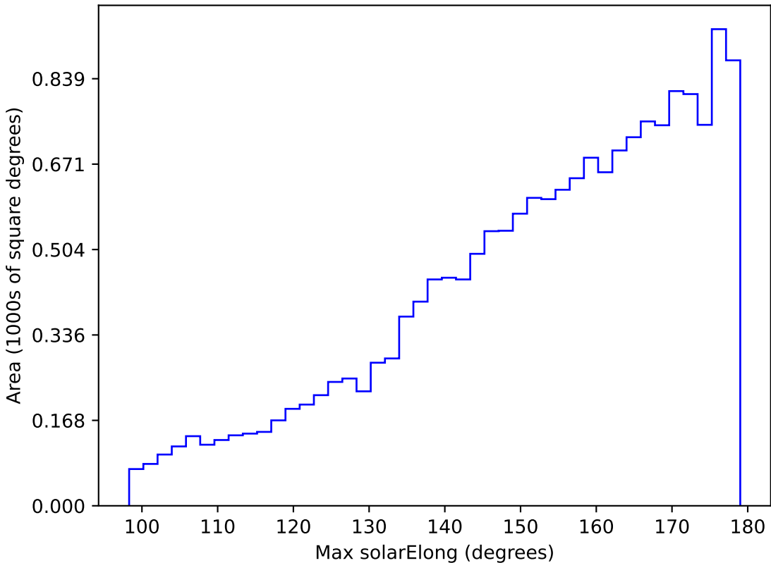
internal_u_expt60_nscale0.9v3.4_10yrs WFD g band: Max solarElong
