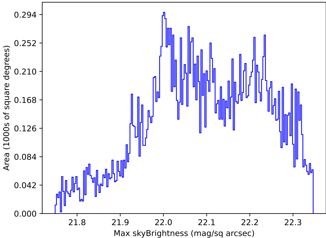
internal_u_expt60_nscale0.9v3.4_10yrs Yr 1 g band: Max skyBrightness
