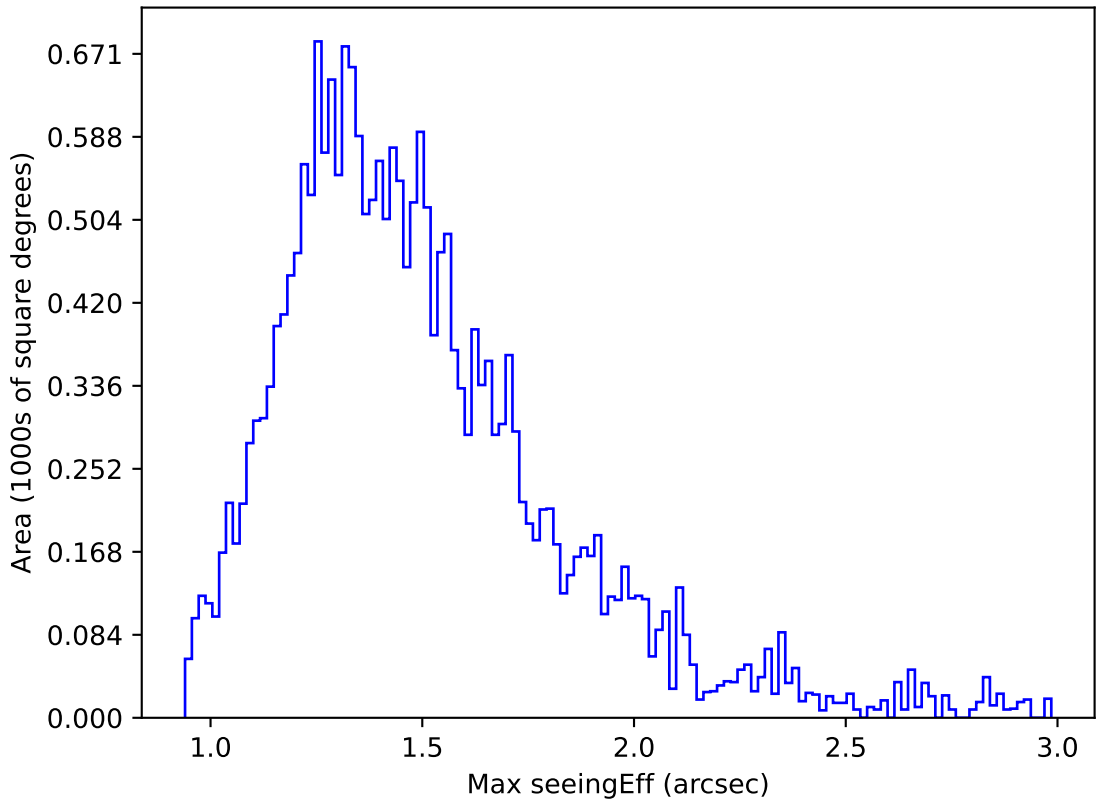
internal_u_expt60_nscale0.9v3.4_10yrs Yr 1 y band: Max seeingEff
