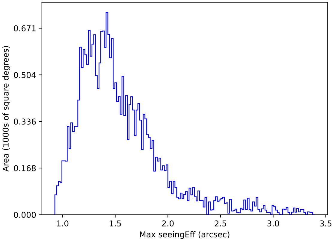
internal_u_expt60_nscale0.9v3.4_10yrs Yr 1 i band: Max seeingEff
