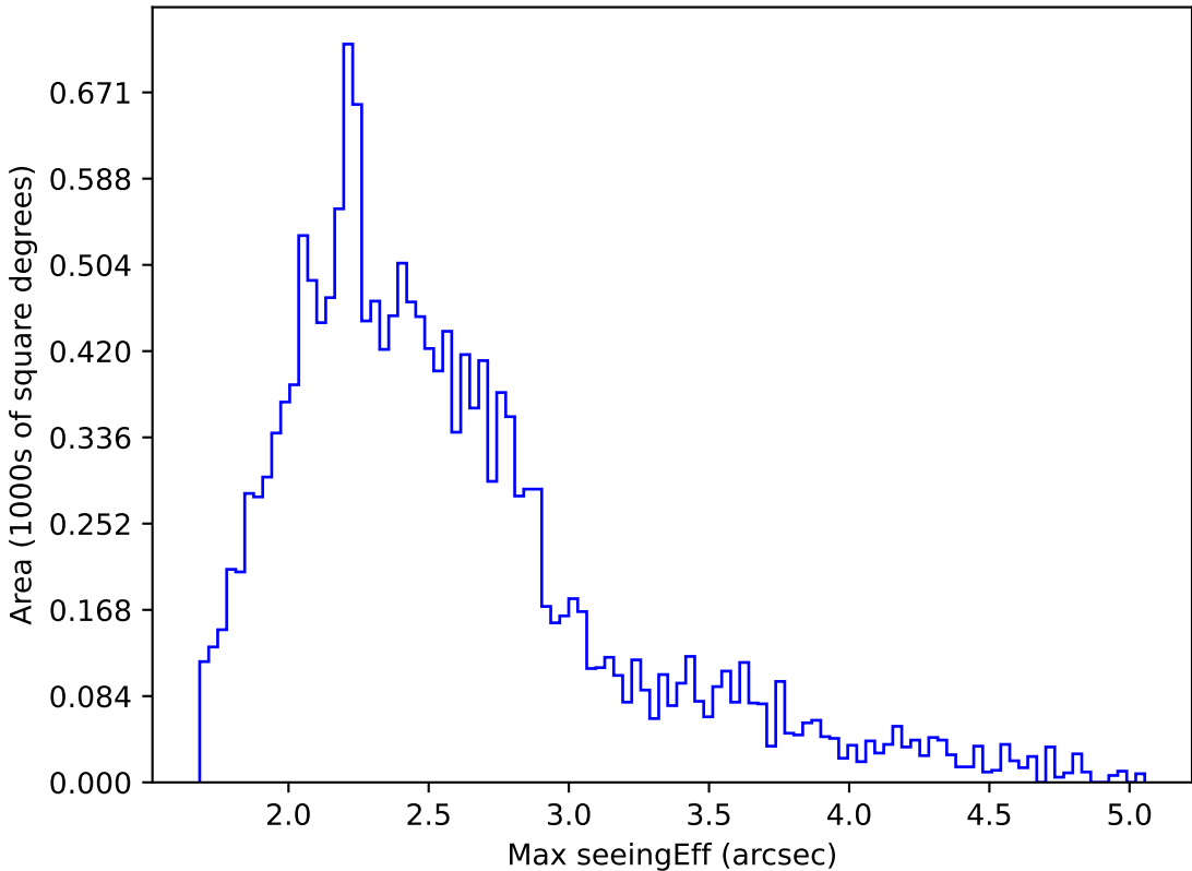
internal_u_expt60_nscale0.9v3.4_10yrs WFD z band: Max seeingEff
