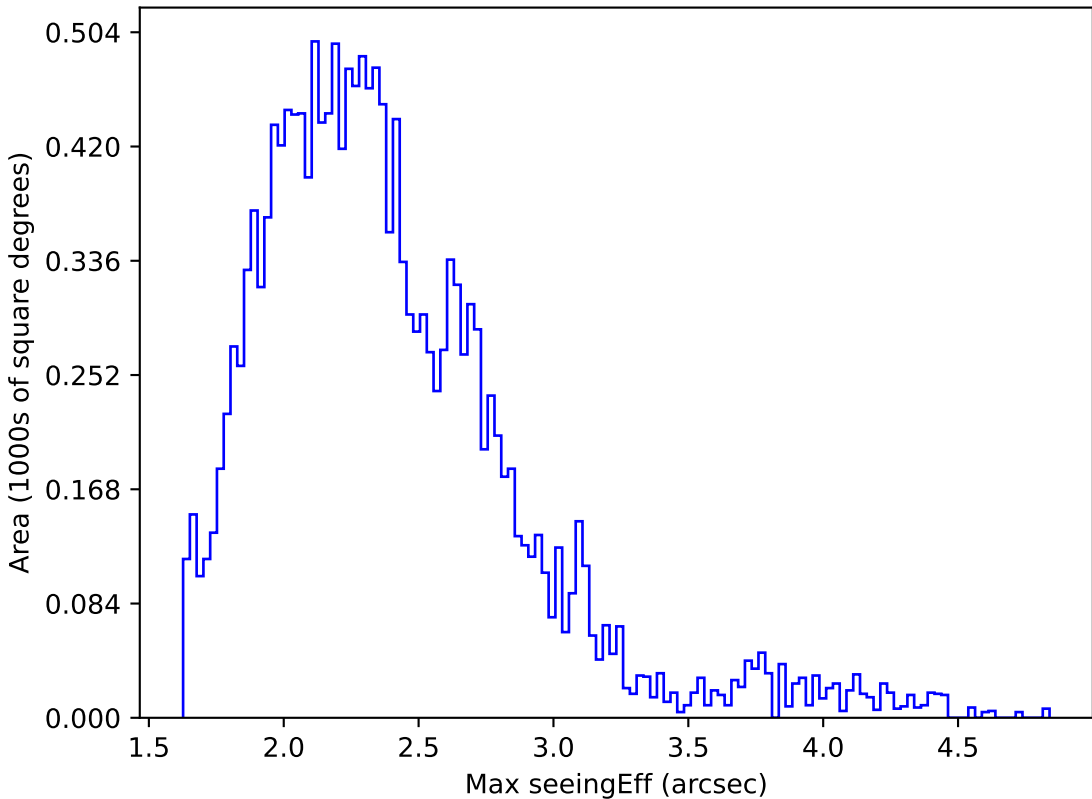
internal_u_expt60_nscale0.9v3.4_10yrs WFD y band: Max seeingEff
