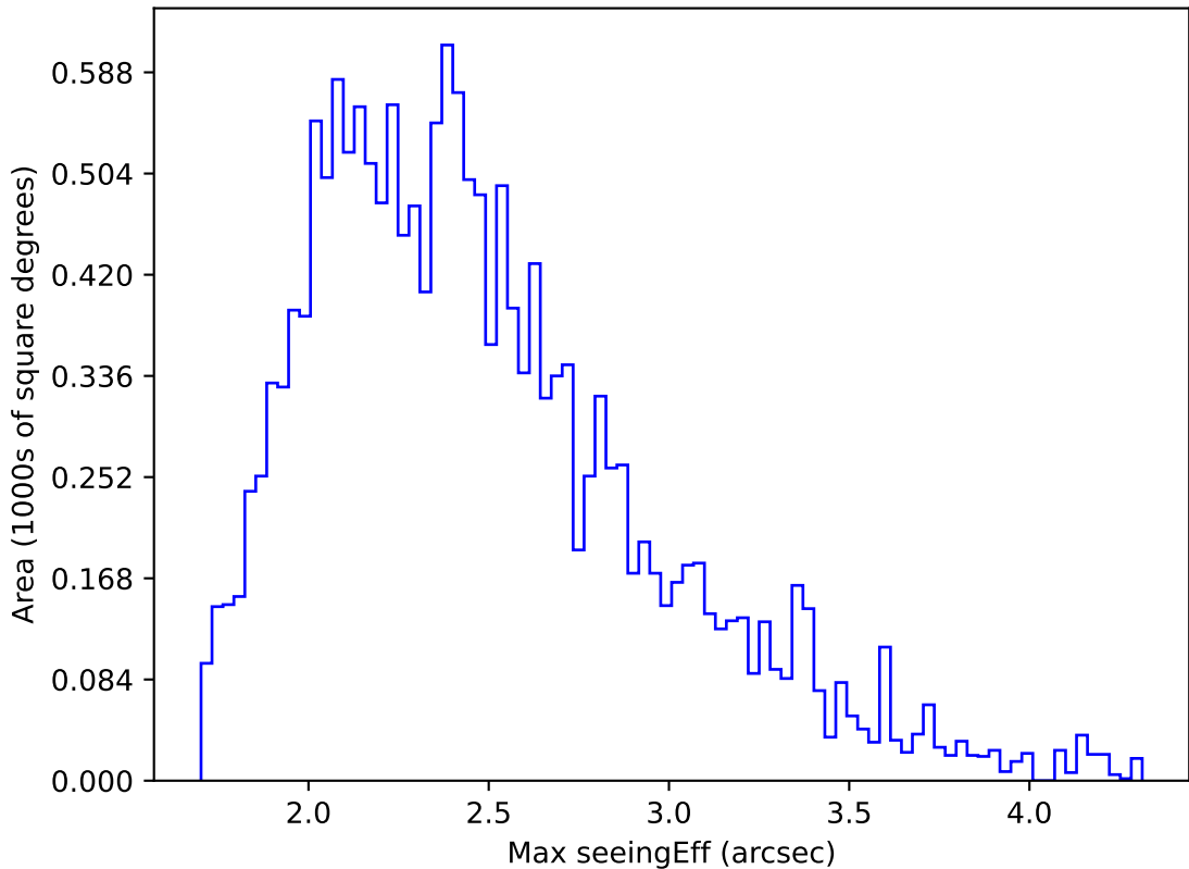
internal_u_expt60_nscale0.9v3.4_10yrs WFD u band: Max seeingEff
