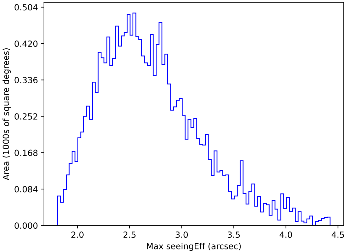
internal_u_expt60_nscale0.9v3.4_10yrs WFD r band: Max seeingEff
