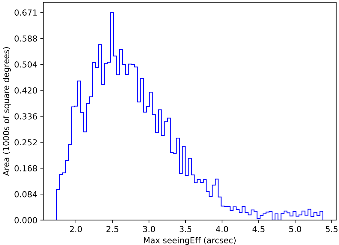
internal_u_expt60_nscale0.9v3.4_10yrs WFD i band: Max seeingEff
