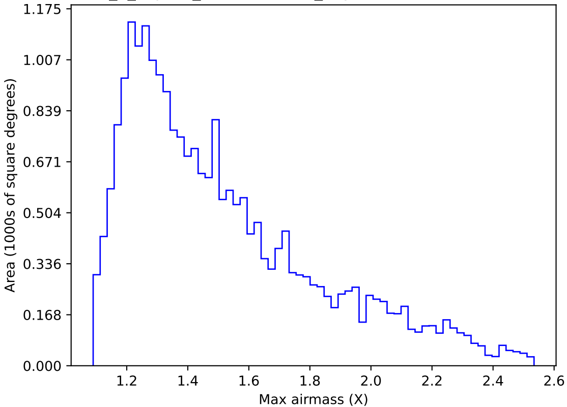
internal_u_expt60_nscale0.9v3.4_10yrs Yr 1 u band: Max airmass
