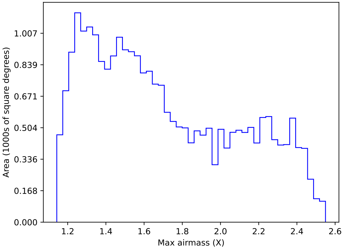
internal_u_expt60_nscale0.9v3.4_10yrs Yr 1 r band: Max airmass
