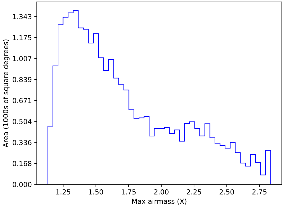
internal_u_expt60_nscale0.9v3.4_10yrs Yr 1 i band: Max airmass
