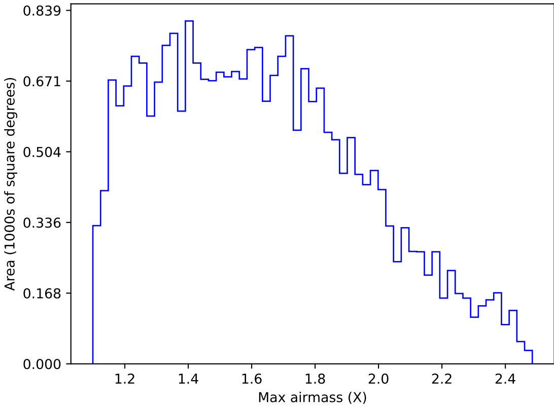
internal_u_expt60_nscale0.9v3.4_10yrs Yr 1 g band: Max airmass
