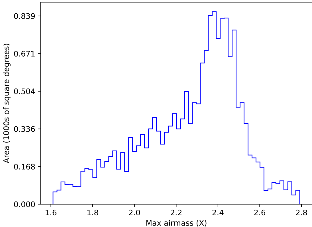
internal_u_expt60_nscale0.9v3.4_10yrs WFD r band: Max airmass
