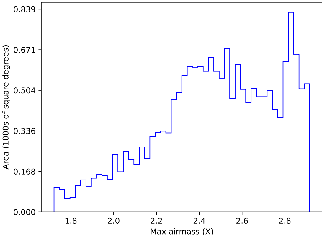
internal_u_expt60_nscale0.9v3.4_10yrs WFD i band: Max airmass
