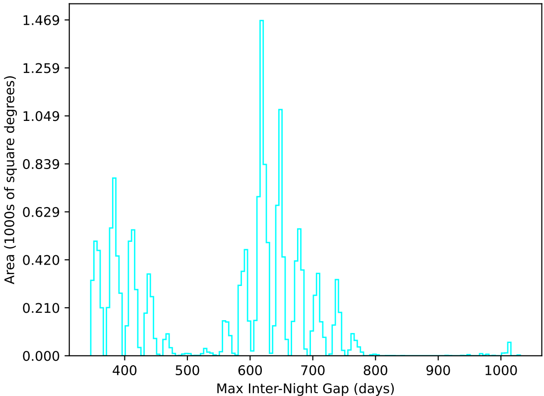
internal_u_expt60_nscale0.9v3.4_10yrs WFD u band: Max Inter-Night Gap
