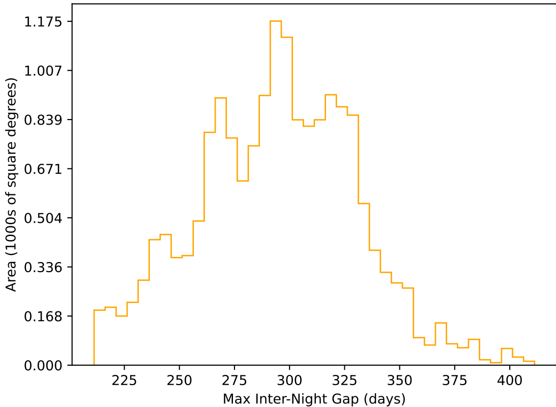
internal_u_expt60_nscale0.9v3.4_10yrs WFD r band: Max Inter-Night Gap
