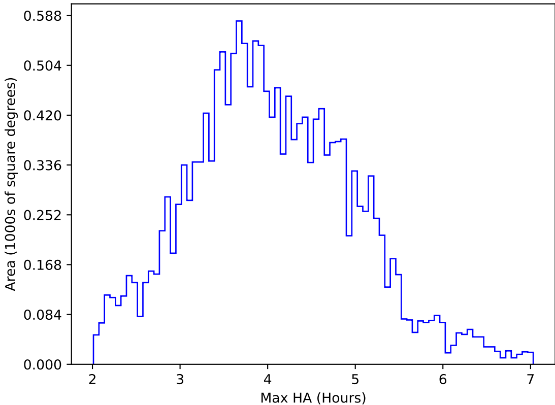
internal_u_expt60_nscale0.9v3.4_10yrs WFD u band: Max HA
