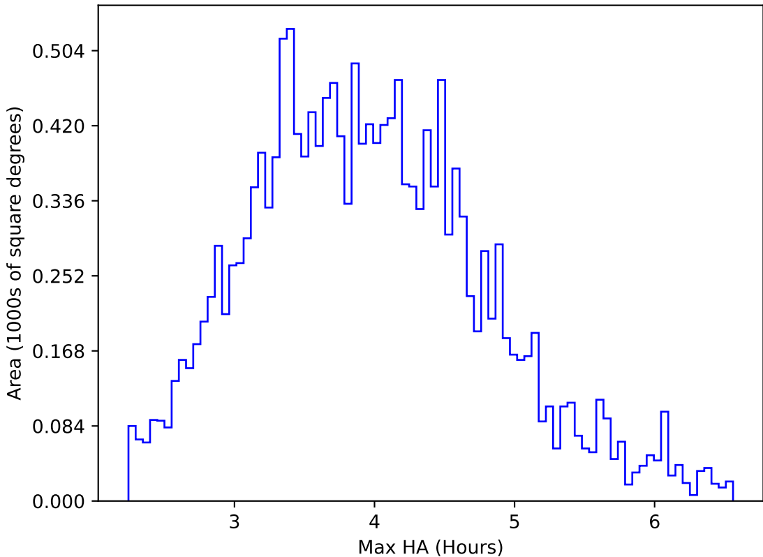
internal_u_expt60_nscale0.9v3.4_10yrs WFD g band: Max HA
