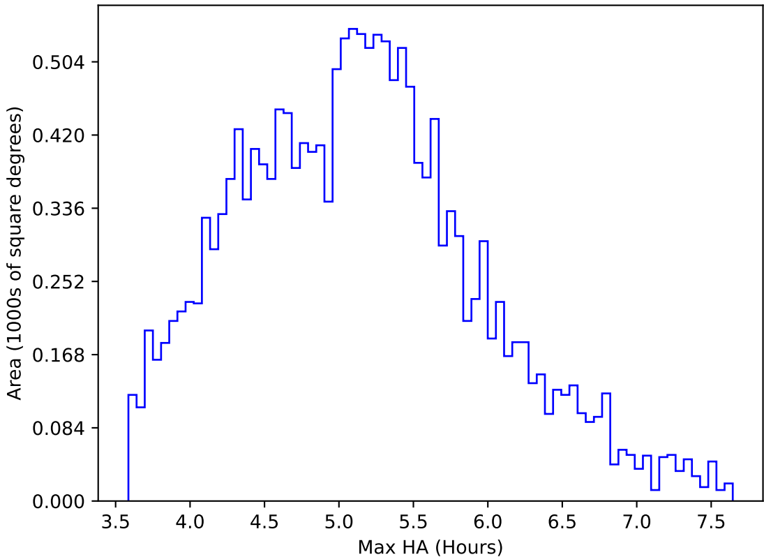
internal_u_expt60_nscale0.9v3.4_10yrs WFD all bands: Max HA
