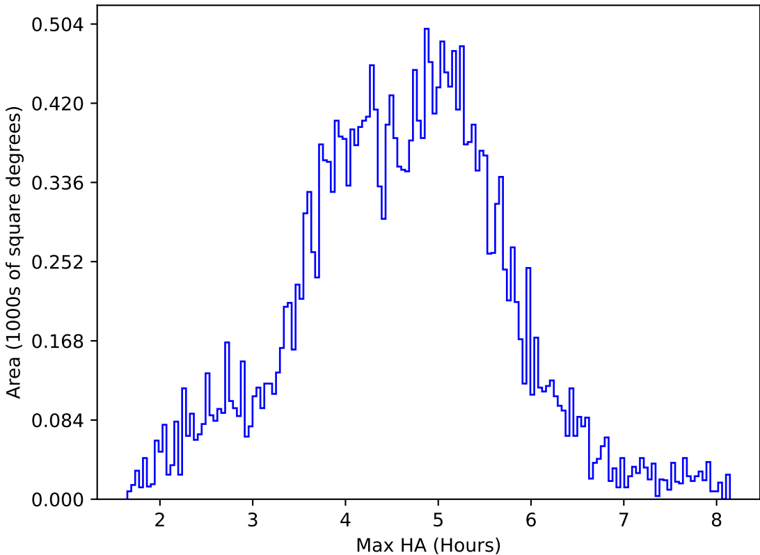
internal_u_expt60_nscale0.9v3.4_10yrs All sky z band: Max HA
