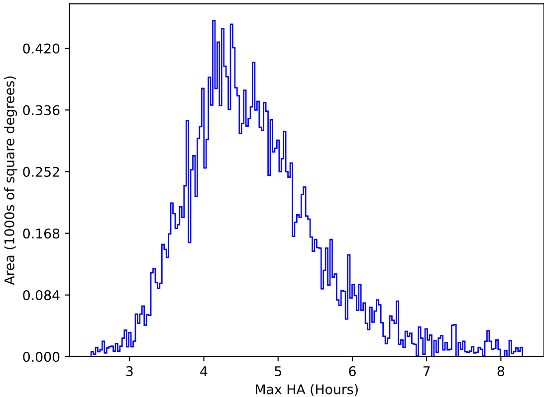
internal_u_expt60_nscale0.9v3.4_10yrs All sky y band: Max HA
