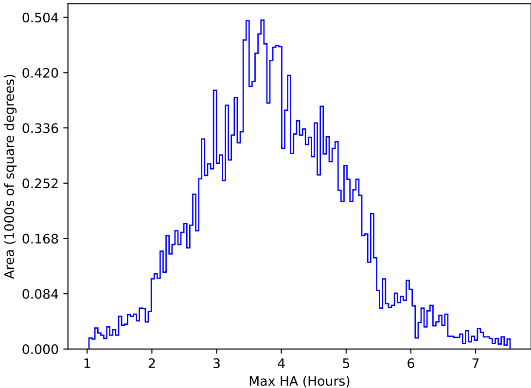
internal_u_expt60_nscale0.9v3.4_10yrs All sky u band: Max HA
