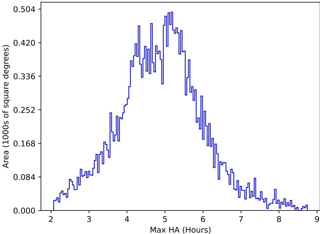
internal_u_expt60_nscale0.9v3.4_10yrs All sky all bands: Max HA
